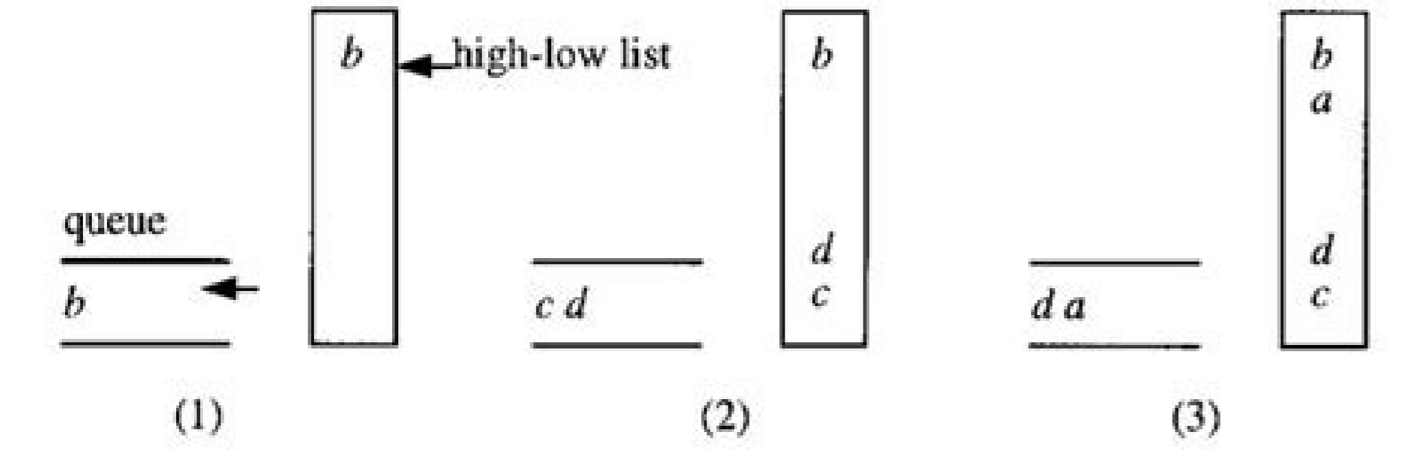
(b) The contents in the queue and the high-low list after: (1) b is selected as the initial extreme vertex and marked high; (2) b is processed ( b is deleted from the braces \{a, b\} and \{b, c\} ); (3) c is processed.
